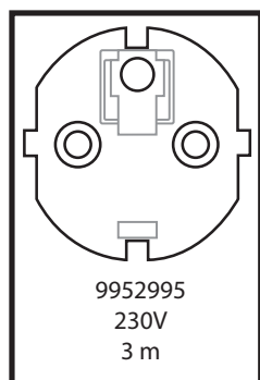
CEE 7/7
